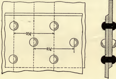
FIG. 42.—TRIPLE-RIVETED JOINT.
